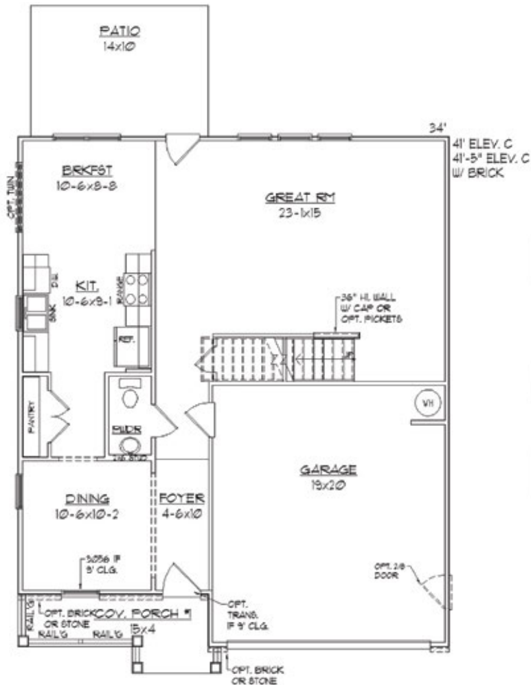
FIRST FLOOR PLAN C
