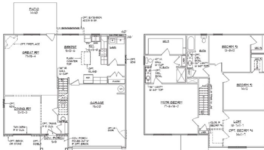
FIRST FLOOR PLAN A & B
