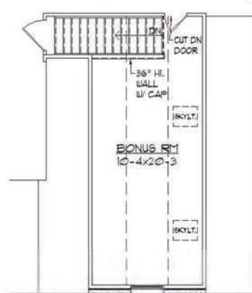
SECOND FLOOR B - OPT. BONUS NOTE: BONUS RM NOT OFFERED FOR ELEV. A
