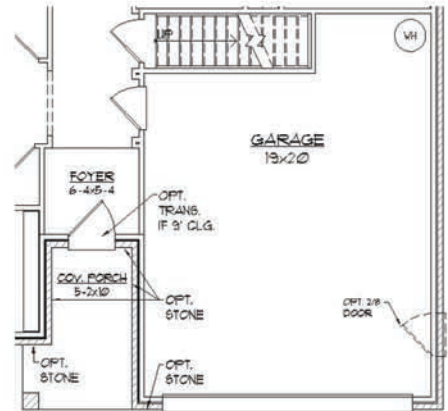
FIRST FLOOR B - OPT. BONUS NOTE: BONUS RM NOT OFFERED FOR ELEV. A
