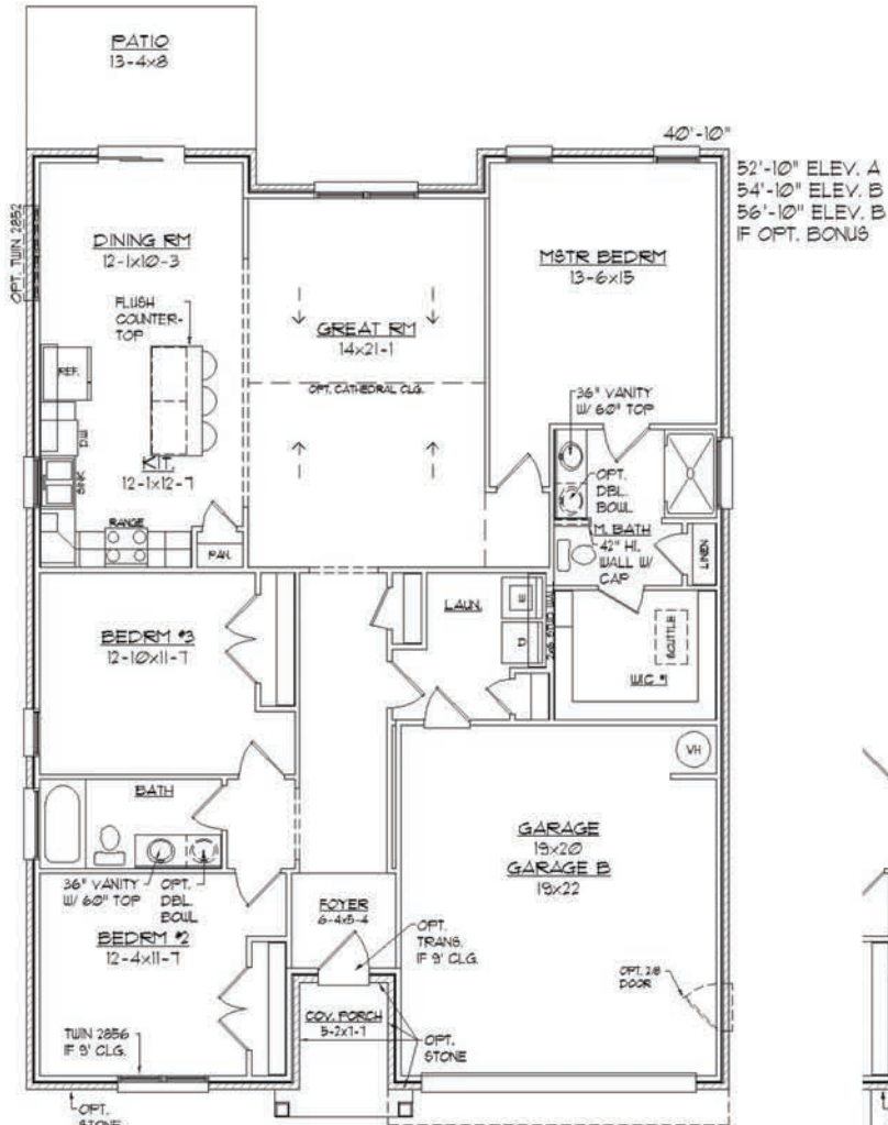
FIRST FLOOR PLAN A OPT. FULL BRICK
