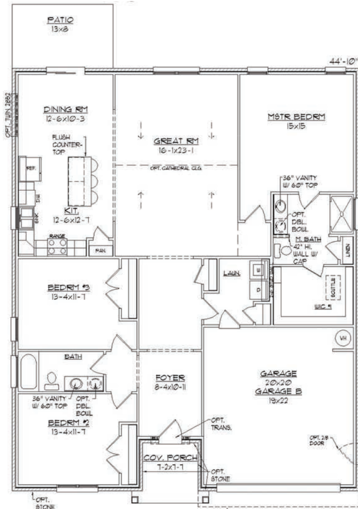
FIRST FLOOR PLAN A OPT. FULL BRICK
