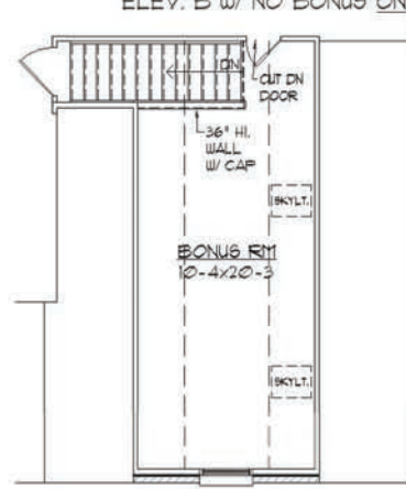
SECOND FLOOR B - OPT. BONUS NOTE: BONUS RM NOT OFFERED FOR ELEV. A
