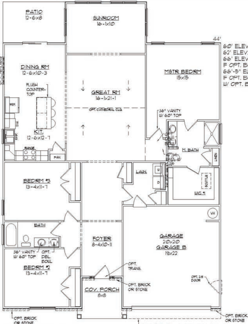
FIRST FLOOR PLAN A NOTE: SEE ELEVATIONS WHERE BRICK OR STONE IS BEING OFFERED.
